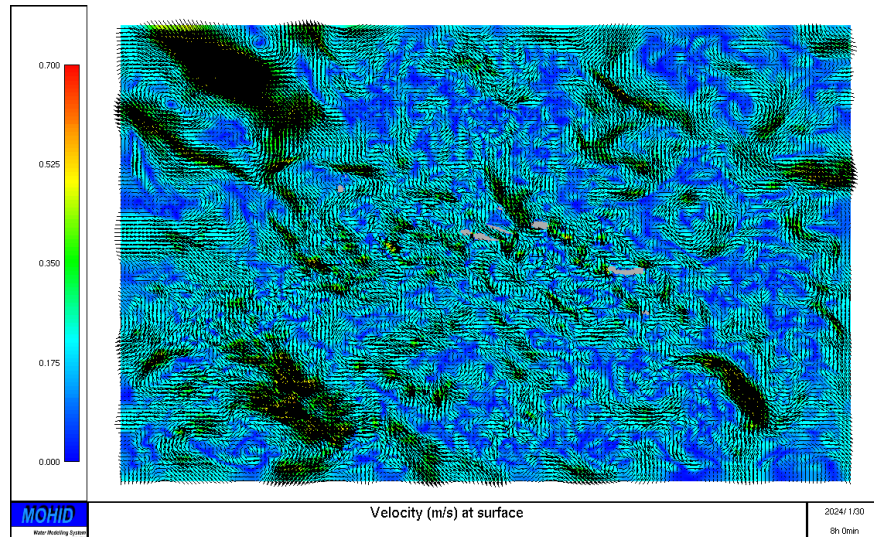
Figure 12 - Example of results obtained for surface velocity for the area of Azores
